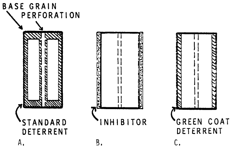
Figure 1. Examples of Deterrent- and Inhibitor-Treated Propellants
