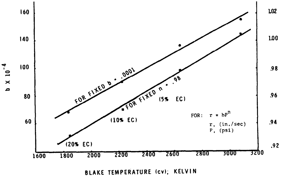
Figure 8. Correlation of Moy Burning Rate Data, Ref 8, with Flame Temperature with Both a Constant Exponent, N, and Coefficient b
