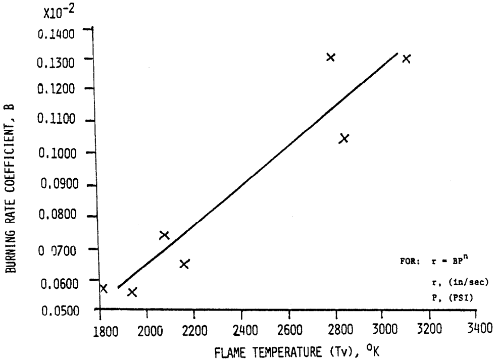
Figure 7. Correlation of Riefler and Lowery Burning Rate Data, Ref. 13, with Flame Temperature by Stiefel, Ref. 7.
