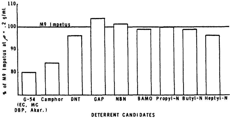
Figure 11. Impetus of M9 with Various Deterrents at a 20% Concentration
