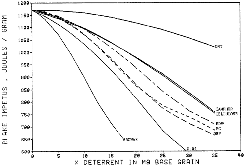
Figure 5. Plot of Change in Impetus of Selected Deterrents from Table II in an M9 Base Grain
