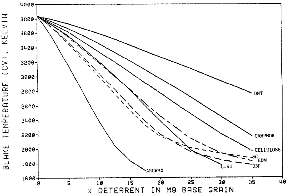
Figure 6. Plot of Change in Isocloric Adiabatic Flame Temperature of Selected Deterrents from Table II in an M9 Base Grain
