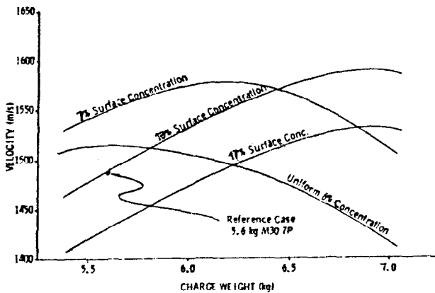
Figure 9. Predicted Velocity of Deterred High-Energy 19-Perforation Propellant with Varying Deterrent Levels ( P_{max} = 415 \text{ MPa} ) (Reference 3)
