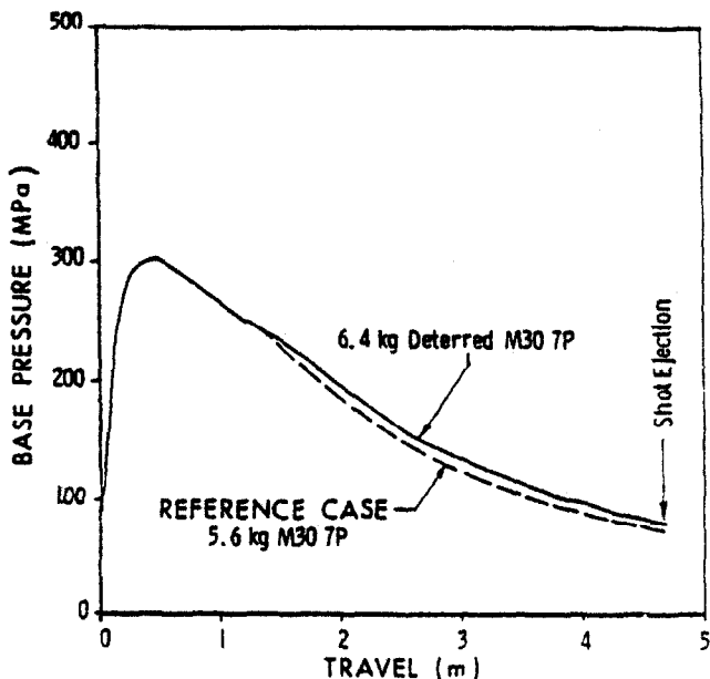
Figure 3. Base Pressure vs Travel with Standard and Deterred M30 7P Propelling Charges (Reference 3)
