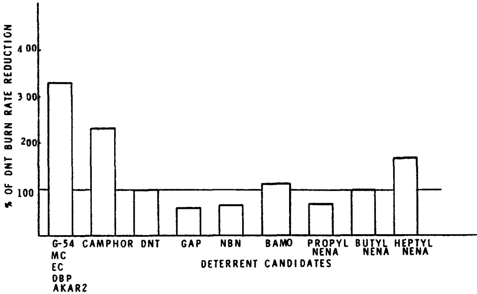
Figure 10. Predicted Burn Rate Reduction of M9 with Various Deterrents (20% Deterrent Concentration)
